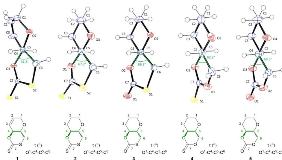
Fig. 2 ORTEP drawings of the crystal structure of 1–5 with thermal ellipsoids at the 50% probability level (see ESI†). For each crystal structure the \text{O}\text{--C}^4\text{--C}^5\text{--C}^6 torsion angle is drawn and highlighted in the accompanying structures below. Single crystals were obtained for each monomer by layering chloroform with n -hexane.
