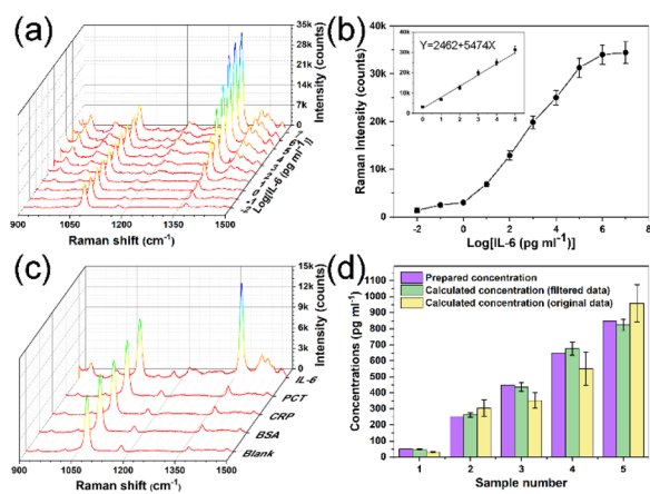
Fig. 5 (a) Average Raman spectra of different concentrations of IL-6 from 10 \text{ fg mL}^{-1} up to 10 \text{ }\mu\text{g mL}^{-1} . (b) Reference plot of the Raman intensity at 1370 \text{ cm}^{-1} vs. the logarithm of IL-6 concentrations with the error bar calculated from filtered signals (The inset was the linear part of the reference plot.). (c) SERS spectra of IL-6 ( 100 \text{ pg mL}^{-1} ), PCT ( 10 \text{ ng mL}^{-1} ), 10 \text{ ng mL}^{-1} CRP ( 10 \text{ ng mL}^{-1} ) and BSA ( 0.5 \text{ mg mL}^{-1} ). (d) Five prepared concentrations of IL-6 in human serum and their corresponding calculated values. (All error bars were calculated from ten repeats.)
