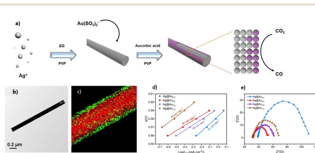
Fig. 4 (a) Schematic preparation process of Ag@Au core-shell nanowires. (b) Representative TEM image. (c) HAADF-STEM elemental mapping. (d) Tafel slope of Ag@Au 0.2 , Ag@Au 0.5 , Ag@Au 0.8 and Ag@Au 1 electrocatalysts. (e) EIS characterization of Ag@Au 0.2 , Ag@Au 0.5 , Ag@Au 0.8 and Ag@Au 1 electrocatalysts.
