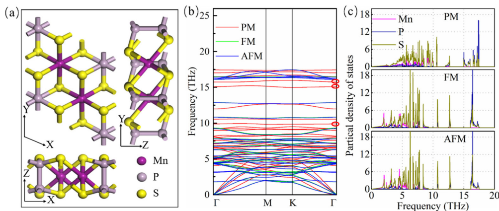
Fig. 1 The structure and phonon behaviors. (a) Atomic structure of monolayer MnPS 3 . (b) Phonon dispersions and (c) phonon density of states of monolayer MnPS 3 with PM/FM/AFM phases.
