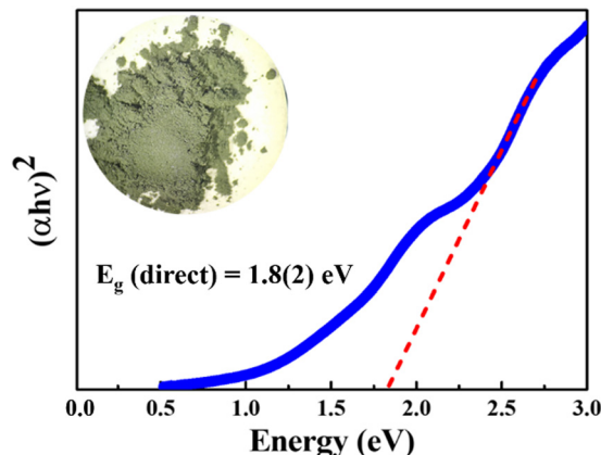
Fig. 4 The solid-state direct bandgap Tauc plot for the polycrystalline BaCeCuS 3 sample.
