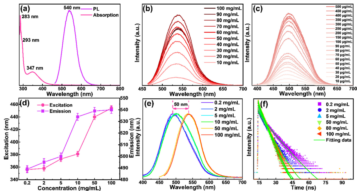
Fig. 3 (a) The absorption and emission spectra of the yellow emitting CDs dispersed in ethanol solution. (b) The PL spectra of the yellow emitting CDs under different concentrations at an excitation wavelength of 454 nm. (c) The PL spectra of the yellow emitting CDs under lower concentrations at an excitation wavelength of 454 nm. (d) The relationship between excitation and emission at different concentrations. (e) Optimum PL spectra of the CDs with different concentrations from 0.2 to 100 mg mL -1 . (f) The corresponding time-resolved PL decay curves.
