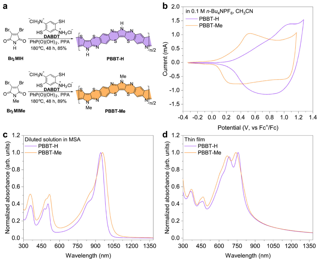
Fig. 1 Synthesis and physicochemical properties of PBBT-H and PBBT-Me. (a) Synthetic route of PBBT-H and PBBT-Me. (b) CV of PBBT-H and PBBT-Me in 0.1 M n\text{-Bu}_4\text{NPF}_6 acetonitrile solution. (c) and (d) UV-vis-NIR absorption spectra of PBBT-H and PBBT-Me in diluted MSA solutions (c) and thin films (d).
