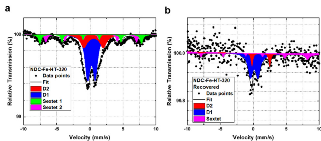
Fig. 5 Mössbauer spectra of NDC-Fe-HT-320 measured at 4.2 K (a) before and (b) after thermal recovery.
