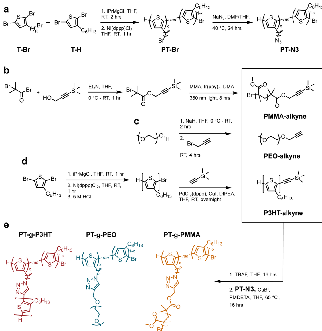
Scheme 1 (a) Synthesis of polythiophene backbone through Kumada coupling and nucleophilic S N 2 substitution (b) synthesis of PMMA side chains through light-mediated ATRP (c) synthesis of alkyne-terminated poly(ethylene oxide) through S N 2 substitution (d) synthesis of P3HT side chains through Kumada coupling and alkyne addition with a Songashira coupling (e) grafting-to approach using CuAAC and graft polymer chemical structures.
