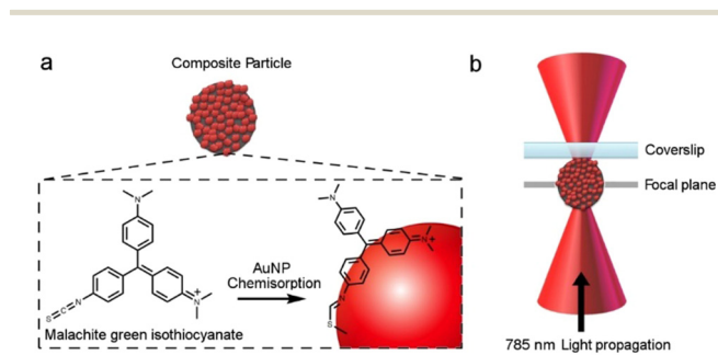
Fig. 4 (a) Representation of MG adsorption at the AuNP surface. (b) Schematic of metal coated dielectric particle pinned close to a surface by a tightly focused laser beam.
