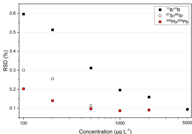
Fig. 1 Isotope ratio precision of ^{11}\text{B}/^{10}\text{B} , ^{87}\text{Sr}/^{86}\text{Sr} and ^{208}\text{Pb}/^{206}\text{Pb} , expressed as RSD (%), for an acquisition time of 10 s per run ( M ) and M = 20 , obtained for different elemental mass concentrations. The data shown are from the measurement of a mixture in which B, Sr, and Pb were detected simultaneously.
