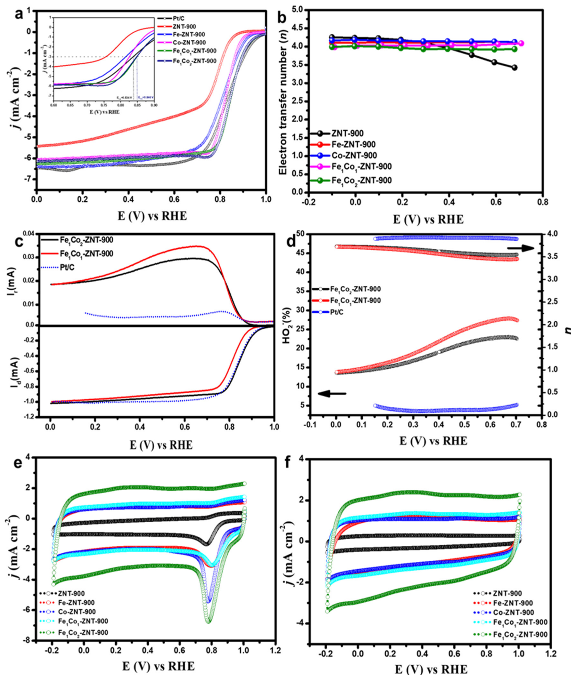
Fig. 6 (a) ORR polarisation curves for ZIF@CNT catalysts recorded at 1900 rpm with a scan rate of 10 \text{mV s}^{-1} in \text{O}_2 -saturated 0.1 M KOH. (b) Electron transfer number ( n ) obtained from K-L plots for all the catalysts. (c) RRDE results for \text{Fe}_1\text{Co}_2 -ZNT-900, \text{Fe}_1\text{Co}_1 -ZNT-900 and Pt/C catalysts in 0.1 M KOH at 1900 rpm with a scan rate of 10 \text{mV s}^{-1} . (d) Electron transfer number ( n ) and \text{HO}_2^- yield for \text{Fe}_1\text{Co}_2 -ZNT-900, \text{Fe}_1\text{Co}_1 -ZNT-900 and Pt/C catalysts. CV curves were recorded in (e) \text{O}_2 -saturated and (f) Ar-saturated 0.1 M KOH at 100 \text{mV s}^{-1} .
