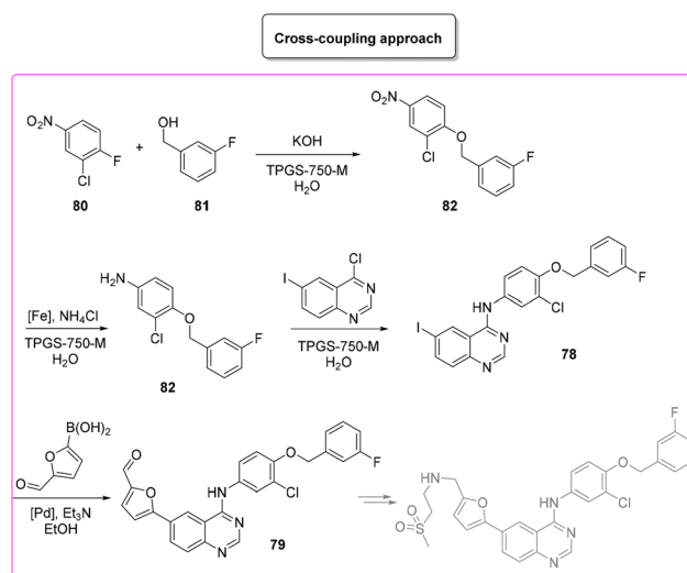
Scheme 37 Lapatinib synthesis via cross-coupling.
