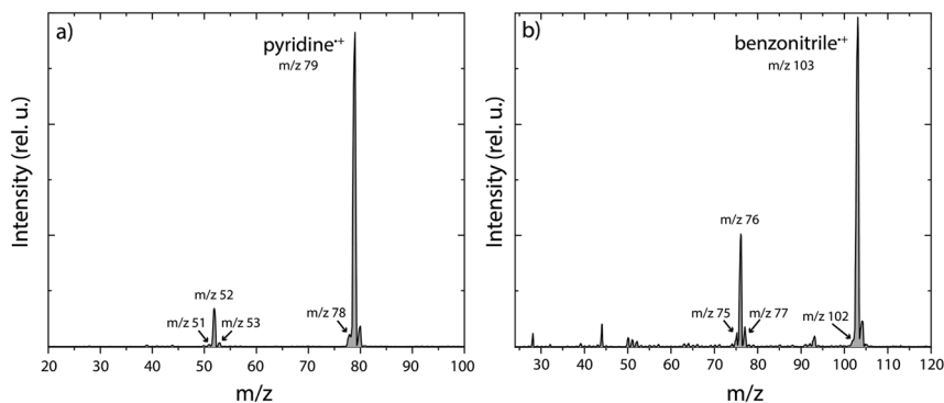
Fig. 1 Experimental mass spectra of the dissociative ionization of (a) pyridine and (b) benzonitrile at an electron impact energy of 15\ \text{eV} . The fragments that are studied in this paper are labelled with their m/z value.
