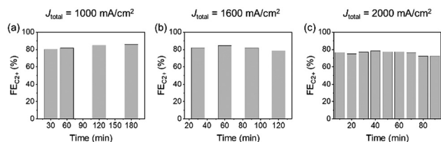
Fig. 5 \text{FE}_{\text{C}_{2+}} stability tests with respect to the current density over CuONPs-1.0/GDE in 1 M KCl under (a) J_{\text{total}} = 1000 mA cm -2 , (b) 1600 mA cm -2 and (c) 2000 mA cm -2 .
