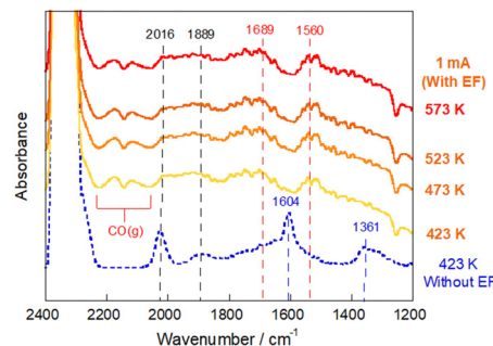
Fig. 6 In situ DRIFTS spectra under the RWGS reaction atmosphere over the Ru(c)/ZrTiO 4 catalyst recorded before/during application of the electric field (EF) at 423–573 K; CO 2 :H 2 :Ar = 1:1:2; 40 SCCM total flow rate.
