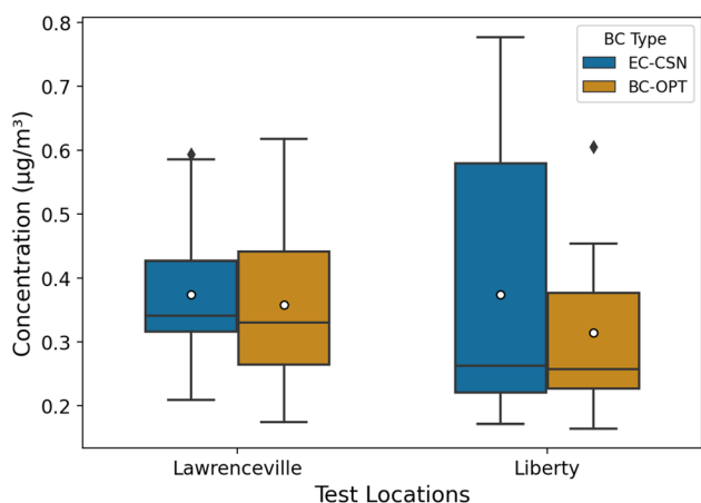
Fig. 5 The boxplot is a comparison of the daily average BC-OPT with EC-CSN in Pittsburgh, Pennsylvania. Lawrenceville CSN site (AQ5 ID: 42-003-0008) measures EC 1-in-3 days, whereas the frequency is every 6 th day in Liberty (AQ5 ID: 42-003-0064). In this plot, we compare daily average BC values at the two sites for 19 and 13 days, respectively. The boxes show the interquartile range and whiskers on the two ends extend to 1.5 times the interquartile range. The data points outside the whiskers are considered outliers. The white dots in the boxes represent mean values.
