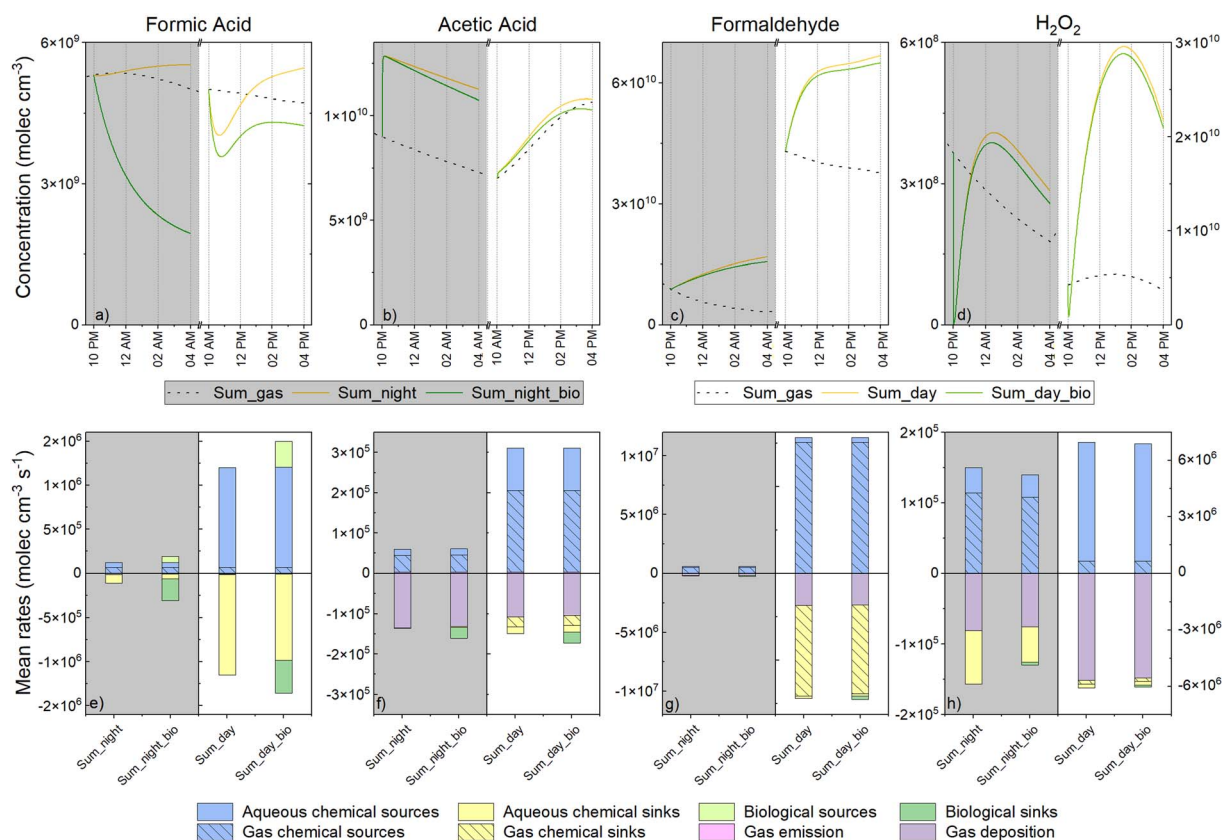
Fig. 6 Total concentration (top) and total chemical budget (bottom) of the four compounds (formic and acetic acids, formaldehyde and H 2 O 2 ) used in simulations. The total concentration is the sum (in molecules cm -3 ) of the aqueous and the gas phase concentrations of different simulations with (green) and without (yellow) consideration of biodegradation. The total chemical budget considers the aqueous transformations: chemical sinks (yellow) and sources (blue) and biodegradation (green); and the gas phase transformations: the chemical sinks (hatched yellow) and sources (hatched blue) as well as the emission (pink) and deposition (purple) processes. The mass transfer was zero as it balanced between the gas and the aqueous phase.
