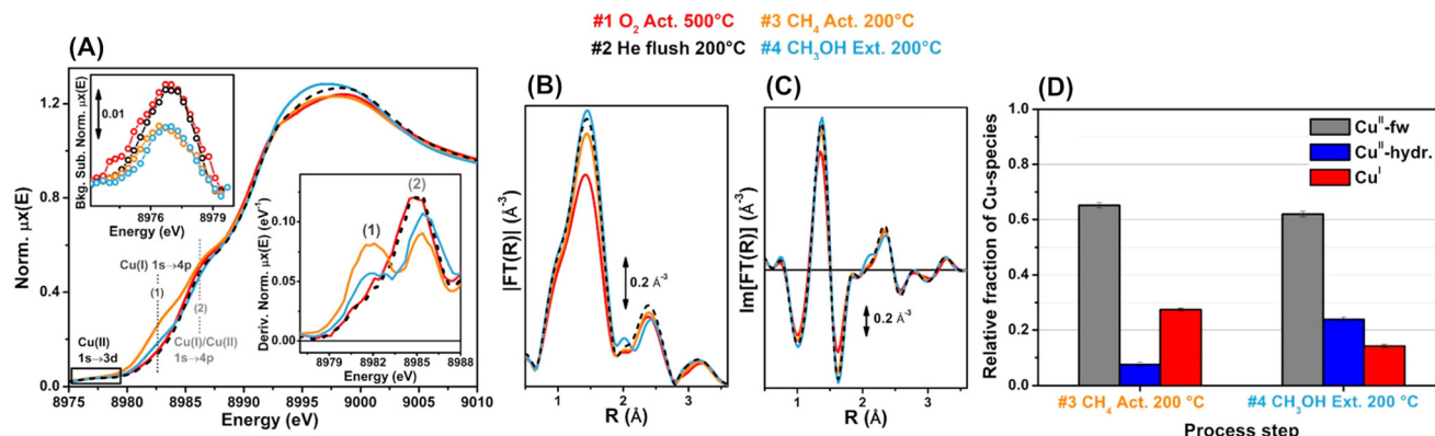
Fig. 25 Operando Cu K-edge XAS spectra of Cu-SSZ-13 after sequential treatments: step 1 (red) = \text{O}_2 activation at 773 K; step 2 (black) = He flushing after cooling to 473 K in \text{O}_2 ; step 3 (orange) = \text{CH}_4 treatment at 473 K; step 4 (blue) = \text{H}_2\text{O} -assisted extraction of methoxy species produced on the catalyst. (A) X-ray absorption near edge structure (XANES) spectra, where labels (1) and (2) represent the rising-edge from 1s to 4p peaks that are characteristic of \text{Cu}^+ and \text{Cu}^+/\text{Cu}^{2+} . (B) Magnitude part of Fourier transform of EXAFS spectra. (C) Imaginary part of Fourier transform of EXAFS spectra. (D) Relative fractions of Cu species estimated via linear combination fitting (LCF) of XANES spectra: \text{Cu}^{\text{II-fw}} = \text{Cu}^{2+} species that interact with the framework; \text{Cu}^{\text{II-hyd.}} = mobile \text{Cu}^{2+} aquo complexes. Reproduced from ref. 109 with permission from American Chemical Society, copyright 2017.
