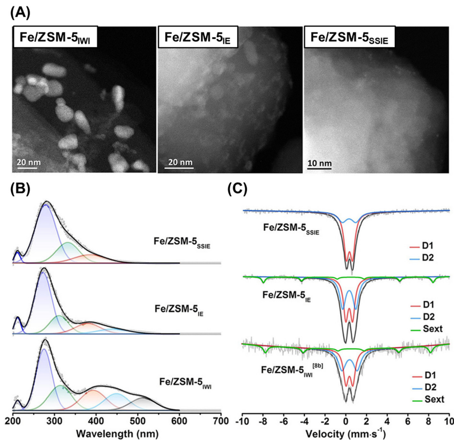
Fig. 15 (A) STEM images, (B) UV-vis spectra, and (C) ^{57}\text{Fe} Mössbauer spectra of Fe/ZSM-5s. Reprinted from ref. 65 with permission from John Wiley and Sons, copyright 2021.
