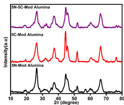
Fig. 9 XRD profile of spent 5Ni-mod alumina, 5C-mod alumina, and 5N-5C-mod alumina catalysts.
