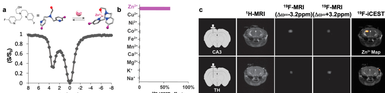
Fig. 7 ^{19}\text{F} -iCEST for mapping labile Zn^{2+} pools. (a) The molecular structure of the ultimate ^{19}\text{F} -iCEST probe designed for mapping labile Zn^{2+} and the obtained ^{19}\text{F} -iCEST effect ( \Delta\omega = 3.2 ppm) of 3 mM probe and 30 \mu\text{M} Zn^{2+} . (b) ^{19}\text{F} -iCEST effect ( \Delta\omega = 3.2 ppm) of 3 mM probe and 30 \mu\text{M} s-block ( Na^+ , K^+ , Mg^{2+} , Ca^{2+} ) and d-block ( Mn^{2+} , Fe^{2+} , Co^{2+} , Ni^{2+} , Cu^{2+} , Zn^{2+} ) metal ions obtained at 37 ^{\circ}\text{C} using a 9.4 T NMR spectrometer. (c) In vivo ^{19}\text{F} -iCEST maps of labile Zn^{2+} pools in the mouse brain. The results are shown for two regions of the brain: CA3 in the hippocampus (zinc-rich ROI, upper row) or the thalamus (TH, zinc-poor ROI, lower row). From left to right are the schematic illustrations of the setup used to deliver a zinc-responsive probe to either CA3 or TH, ^1\text{H} -MRI, ^{19}\text{F} -MRI obtained with saturation pulse applied "off-resonance" ( \Delta\omega = -3.2 ppm), ^{19}\text{F} -MRI obtained with saturation pulse applied "on resonance" ( \Delta\omega = +3.2 ppm), the ^{19}\text{F} -iCEST map ( Zn^{2+} map) obtained from subtracting ^{19}\text{F} -MRI S^{+3.2 \text{ ppm}} from ^{19}\text{F} -MRI S^{-3.2 \text{ ppm}} overlaid on the ^1\text{H} -MRI. Modified with permission from ref. 76.
