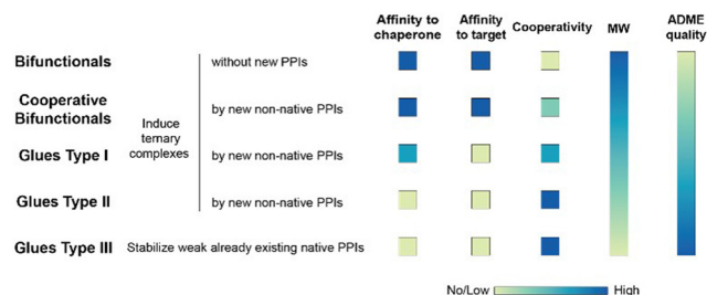
Fig. 1 Ternary complex-forming compounds can be grouped into multiple subtypes by their affinities to one or both proteins that constitute the ternary complex and the degree of induced positive or negative cooperativity. The proposed classification is idealized. In practice, ternary complex-forming compounds are often hybrids of two different types. In ternary complexes with similar thermodynamic stability, the molecular weight of the ternary complex-forming compound should inversely correlate with increasing cooperativity due to additional direct protein–protein or glue–protein interactions, which occur exclusively in the ternary complex. The colour gradient bars for “MW size” and “ADME quality” are intended to qualitatively illustrate the generally acknowledged trend that molecular weight and ADME quality are also inversely correlated ( i.e. , “smaller is better”).
