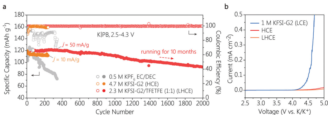
Fig. 1 (a) Cycling performance of K|PB batteries in 0.5 M KPF 6 EC DEC electrolyte at 50\text{ mA g}^{-1} , HCE at 10\text{ mA g}^{-1} , and LHCE at 50\text{ mA g}^{-1} . (b) LSV of various concentrations of KFSI/G2 electrolytes in K|Al coin cells with Al as the working electrode and K metal as the counter electrode. The scan rate is 0.5\text{ mV s}^{-1} .
