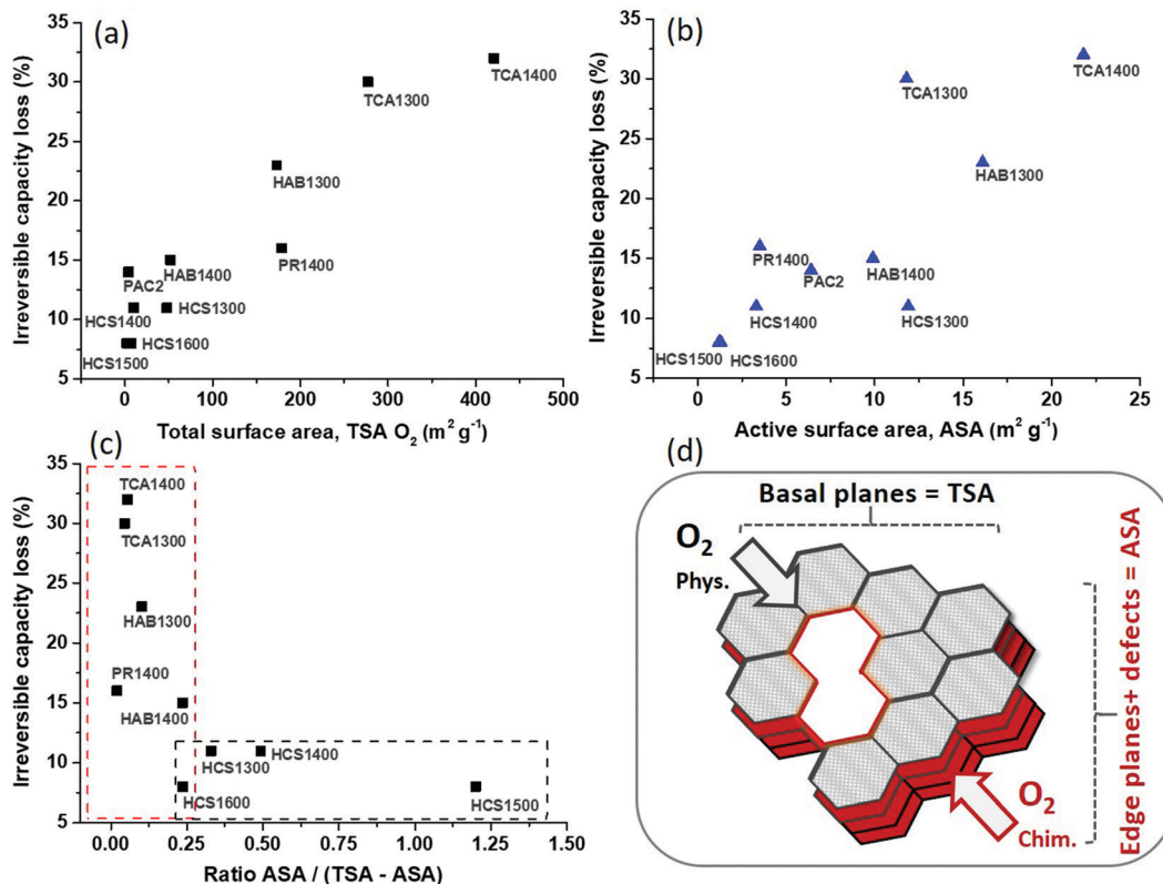
Fig. 3 Relationship between the 1st irreversible capacity loss and (a) total surface area ( TSA_{O_2} ), (b) active surface area (ASA), (c) ratio ASA/(TSA_{O_2}-ASA) . (d) Representation of hard carbon structure containing the active surface (edge planes and defects) and the basal planes surface ( TSA-ASA ).
