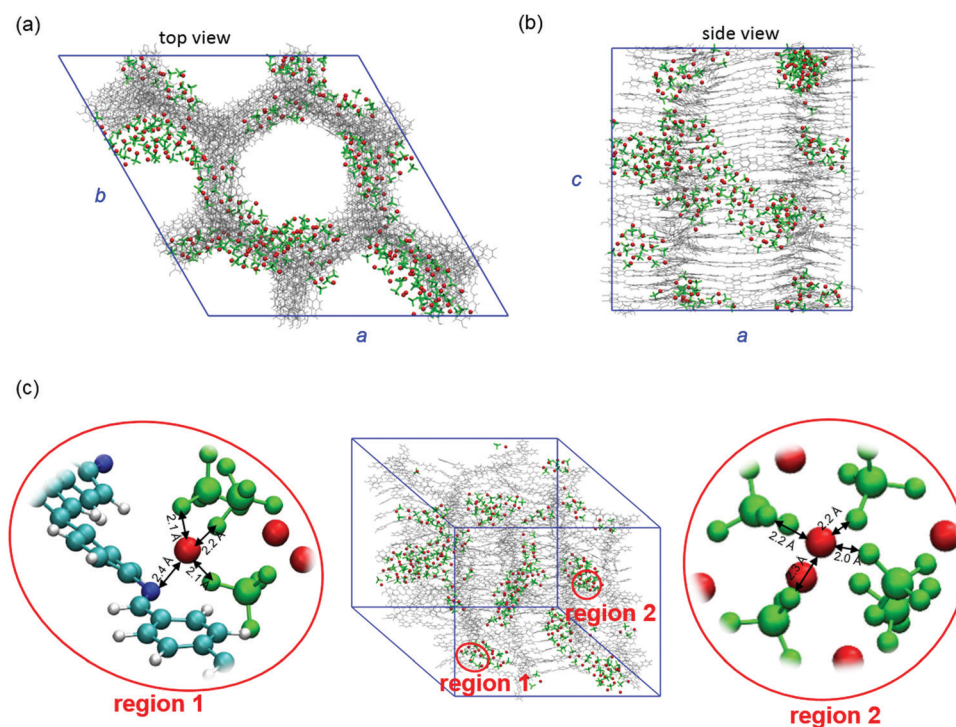
Fig. 2 (a) Top and (b) side view of the snapshot at 200 ns for TAPB-PDA COF mixed with \text{LiClO}_4 . (c) A tilted view of the same structure with representative local structures of \text{Li}^+ , \text{ClO}_4^- , and COF. Red spheres represent \text{Li}^+ . Green spheres and rods represent \text{ClO}_4^- .
