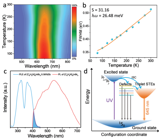
Fig. 5 (a) Temperature-dependent PL spectra measured from 80 to 300 K. (b) Experimental dependence of the FWHM broadening on temperature for (C_6H_8N)_6InBr_9:0.58\%Sb . The FWHM values are fitted with a model, from which the Huang–Rhys factor S is obtained. (c) PL and PLE spectra of (C_6H_8N)_6InBr_9 and (C_6H_8N)_6InBr_9:0.58\%Sb , respectively. (d) Schematic illustration of radiative channels in (C_6H_8N)_6InBr_9:0.58\%Sb .
