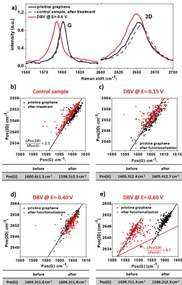
Fig. 4 (a) Raman spectra and (b–e) plots of \text{Pos}(2\text{D}) versus \text{Pos}(\text{G}) of G-SiO 2 samples before and after electrodeposition of DBV. The electrochemical potential at which G-SiO 2 is functionalized by DBV is indicated on top of the panels. The black lines in (b–e) have a slope of 2.2 and highlight the variation in strain and the red guideline in (e) indicates the direction in shift of the data points upon doping.
