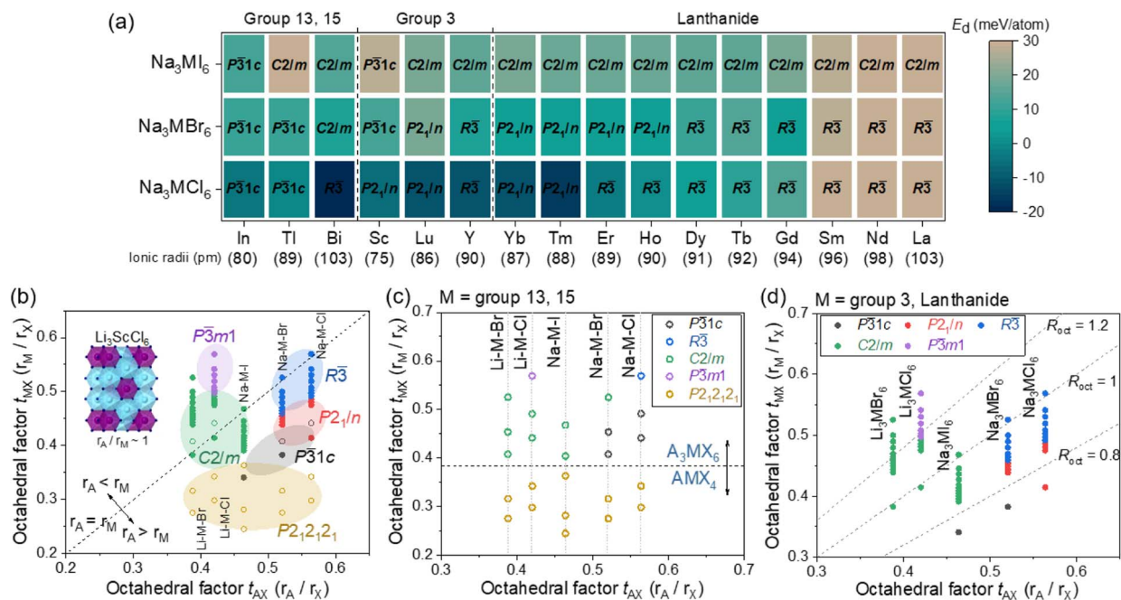
Fig. 1 (a) Heat map for the decomposition energy ( E_d ) of Na halides ( \text{Na}_3\text{MX}_6 , X = \text{Cl} , \text{Br} and \text{I} ) against the competing phases \text{NaX} and \text{MX}_3 . The most stable phase for the crystal structures of P\bar{3}1c , P2_1/n , R\bar{3} , C2/m and P\bar{3}m1 was used to evaluate E_d for \text{Na}_3\text{MX}_6 . (b–d) Structural preference tendencies of the crystal systems for P\bar{3}1c , P2_1/n , R\bar{3} , C2/m , P\bar{3}m1 and P2_12_12_1 as a function of the octahedral factors for \text{AX}_6 ( r_A/r_X ) and \text{MX}_6 ( r_M/r_X ) for Li and Na metal ternary halides based on M elements: (b) all elements, (c) group 13 and 15 elements, (d) group 3 and lanthanide elements. Compounds in same composition group (A–M–X) are aligned vertically in (b–d). R_{\text{Oct}} in (d) corresponds to the ratio of r_A to r_M .
