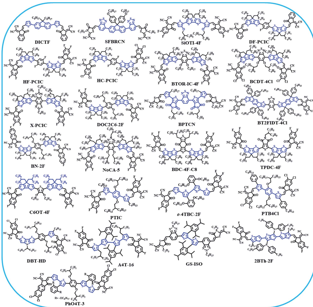
Fig. 4 Chemical structures of unfused-ring small-molecule acceptors.
