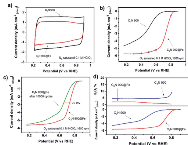
Fig. 4 Cyclic voltammogram of C 2 N 900 before and after Fe metalation recorded at 50 \text{ mV s}^{-1} (a). Capacitance-corrected cathodic scan of the cyclic voltammogram in 0.1 \text{ M HClO}_4 with a rotation speed of 1600 \text{ rpm} recorded at 10 \text{ mV s}^{-1} obtained by subtracting N 2 saturated cyclic voltammetry at 1600 \text{ rpm} from the O 2 saturated result. For C 2 N 900@Fe, three independent measurements were carried out with average value plotted. Error bars correspond to largest deviating value from average at the given potential. (b). Cathodic scans of the cyclic voltammograms at 1600 \text{ rpm} before and after 10\,000 cycles between 0.6 and 0.9 \text{ V} recorded at 100 \text{ mV s}^{-1} under N 2 saturation (c). H 2 O 2 production from cathodic scan RRDE measurement for C 2 N 900 and C 2 N 900@Fe at 1600 \text{ rpm} , 10 \text{ mV s}^{-1} , capacitance correction and under O 2 saturation (d). All measurements conducted with no IR correction, 0.26 \text{ mg cm}^{-2} catalyst loading and room temperature electrolyte.
