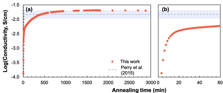
Fig. 10 Plot of conductivity over the full annealing period (a) and over the first hour (b) at 400 °C in ~0.2 atm UHP O 2 and ~0.8 atm UHP Ar; dashed line shows the conductivity and conservative uncertainty estimate (shaded blue) of a crystalline-grown STF35 thin film 26 under the same conditions.
