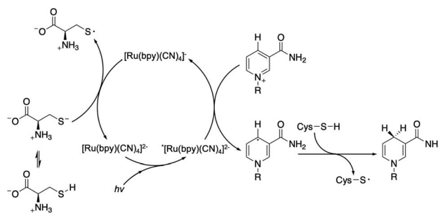
Scheme 2 Proposed mechanism of the photocatalytic cycle for \text{NAD}^\cdot radical formation and its quenching by L -cysteine with the evolution of 1,4-NADH.
