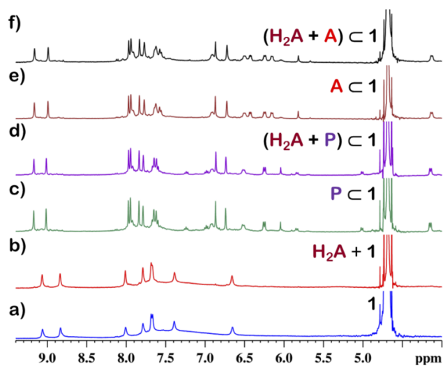
Fig. 6 Partial ^1\text{H} NMR stack plot of (a) 1 , (b) \text{H}_2\text{A} + \mathbf{1} ( \text{H}_2\text{A} = 9,10 -dihydroanthracene), (c) \text{P} < \mathbf{1} ( \text{P} : phenanthrene), (d) (\text{H}_2\text{A} + \text{P}) < \mathbf{1} , (e) \text{A} < \mathbf{1} ( \text{A} : anthracene) and (f) (\text{H}_2\text{A} + \text{A}) < \mathbf{1} in \text{D}_2\text{O} showing the selective encapsulation of A and P .
