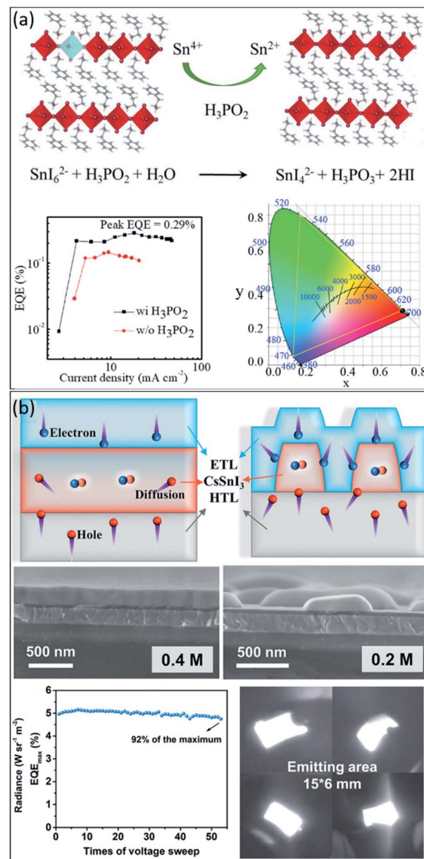
Fig. 7 (a) The proposed mechanism of \text{Sn}^{4+} reduction to \text{Sn}^{2+} using \text{H}_3\text{PO}_2 additive, the EQE versus current density of PeLEDs with and without \text{H}_3\text{PO}_2 , and the corresponding CIE coordinate of the device. 112 Copyright 2020, Wiley. (b) Schematic illustration of the charge carriers transport and recombination in the compact and dendritic \text{CsSnI}_3 Pero-LEDs, cross-sectional SEM images of the structured films with 0.4 M and 0.2 M \text{CsSnI}_3 concentrations, the \text{EQE}_{\text{max}} curve, and photographs of the lighting flexible 0.2 M \text{CsSnI}_3 Pero-LEDs. 148 Copyright 2021, Wiley.
