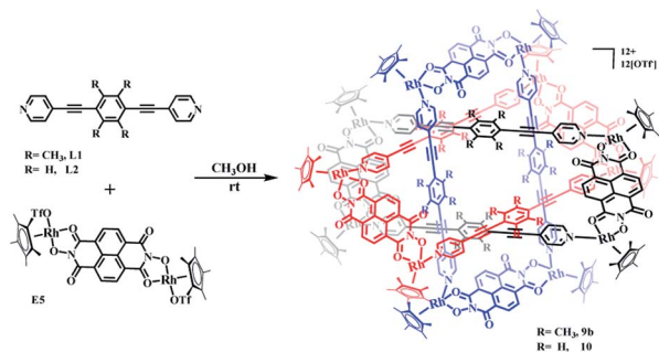
Scheme 3 The synthesis of molecular Borromean ring assemblies 9b and 10 .
