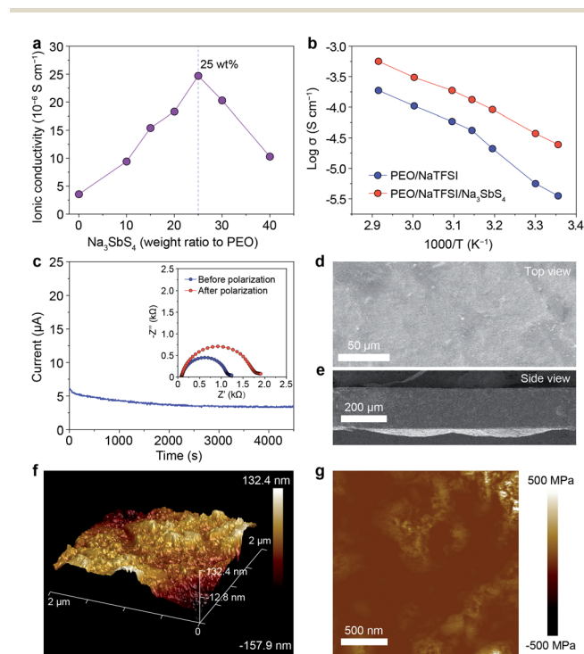
Fig. 2 Characterization of PEO-based all-solid-state electrolytes. (a) Ionic conductivity of the electrolyte with different contents of \text{Na}_3\text{SbS}_4 (calculated based on the mass of PEO). (b) Ionic conductivity of pristine PEO/NaTFSI electrolyte and PEO/NaTFSI/ \text{Na}_3\text{SbS}_4 electrolyte at different temperatures (25, 30, 40, 45, 50, 60, and 70 °C). (c) Variation of current with time for the Na/Na symmetric cell with PEO/NaTFSI/ \text{Na}_3\text{SbS}_4 electrolyte at an applied voltage of 12 mV. Inset: electrochemical impedance spectroscopy (EIS) plots before and after polarization. SEM images of the PEO/NaTFSI/ \text{Na}_3\text{SbS}_4 electrolyte from (d) the top view and (e) side view. (f) AFM topography image with a 3D view and (g) Young's modulus of the PEO/NaTFSI/ \text{Na}_3\text{SbS}_4 electrolyte.
