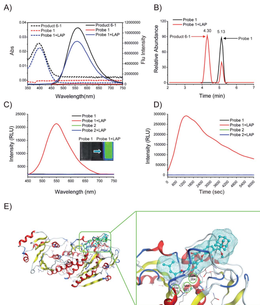
Fig. 3 (A) Absorption (dashed line) and fluorescence (solid line) emission spectra of probe 1. Probe 1 (10 \mu\text{M} ) was incubated with or without LAP (100 U \text{L}^{-1} ) in enzyme assay buffer at 37 ^{\circ}\text{C} for 6 h. (B) HPLC analysis of probe 1 (10 \mu\text{M} ) before (black) and after (red) incubation with LAP (100 U \text{L}^{-1} ) in enzyme assay buffer (pH = 7.4) at 37 ^{\circ}\text{C} for 1 h. (C) Chemiluminescence spectra and images (inset) of probes 1 and 2 (10 \mu\text{M} ). The probes were incubated with or without LAP (100 U \text{L}^{-1} ) at 37 ^{\circ}\text{C} for 10 min. (D) Chemiluminescence kinetic profiles of probes 1 and 2 (10 \mu\text{M} ) after incubation with or without LAP (100 U \text{L}^{-1} ) at 37 ^{\circ}\text{C} for 6000 s. (E) Low-energy binding models of probes 1 (cyan) and 2 (green) bound to the LAP (PDB: 2hc9) interface.
