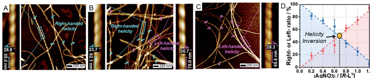
Fig. 2 AFM images of self-assembled R-1^1 with \text{AgNO}_3 obtained in a DMSO and \text{H}_2\text{O} mixture (1 : 1 v/v): (A) 0.0, (B) 0.2, and (C) 1.2 equiv. (D) Plot of the ratio of right- or left-handed helical fibers vs. equivalents of \text{AgNO}_3 . The ratio of right- to left-handed fiber was calculated by the number of individual fibers (50–100); the blue and the red colors indicate the ratio of right- and left-handed fibers, respectively.
