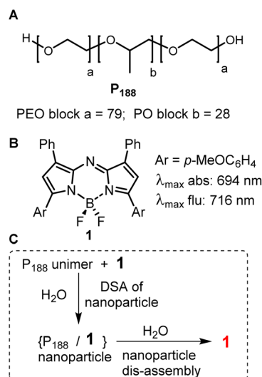
Fig. 1 (A) Structure of PEO/PPO/PEO triblock copolymer P 188 . (B) Structure and spectroscopic characteristics of NIR-AZA fluorophore 1. (C) Directed self-assembly and dis-assembly of P 188 and 1 in water.
