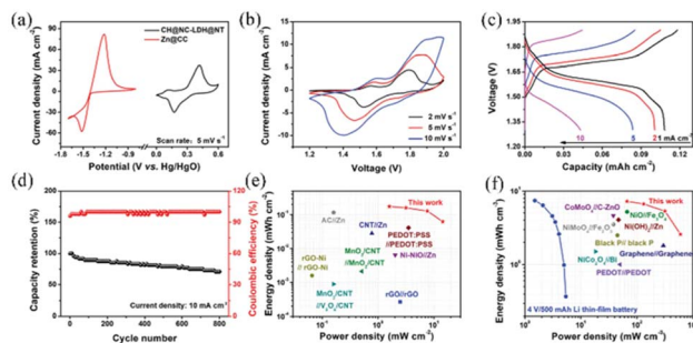
Fig. 5 Electrochemical performances of Co-Zn micro-battery. (a) Cyclic voltammetry (CV) curves of Co(OH) 2 @NiCo-layered double hydroxide@Ni-coated textile and Zn@carbon clothes at 5 mV s -1 . (b) CV curves, (c) galvanostatic charge–discharge (GCD) curves, (d) long-term cycling stability, and (e and f) Ragone plots of Co-Zn micro-battery. 127 Reproduced with permission from ref. 127. Copyright 2020, Wiley.
