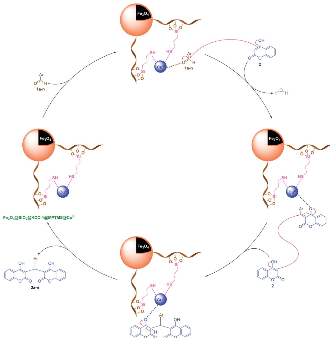
Scheme 5 Plausible mechanism for the solvent-free one-pot pseudo -three-component synthesis of bis-coumarins ( 3a-n ) catalyzed by the \text{Fe}_3\text{O}_4 @ \text{SiO}_2 @ \text{KCC-1} @ \text{MPTMS} @ \text{Cu}^{\text{II}} nanocomposite.
