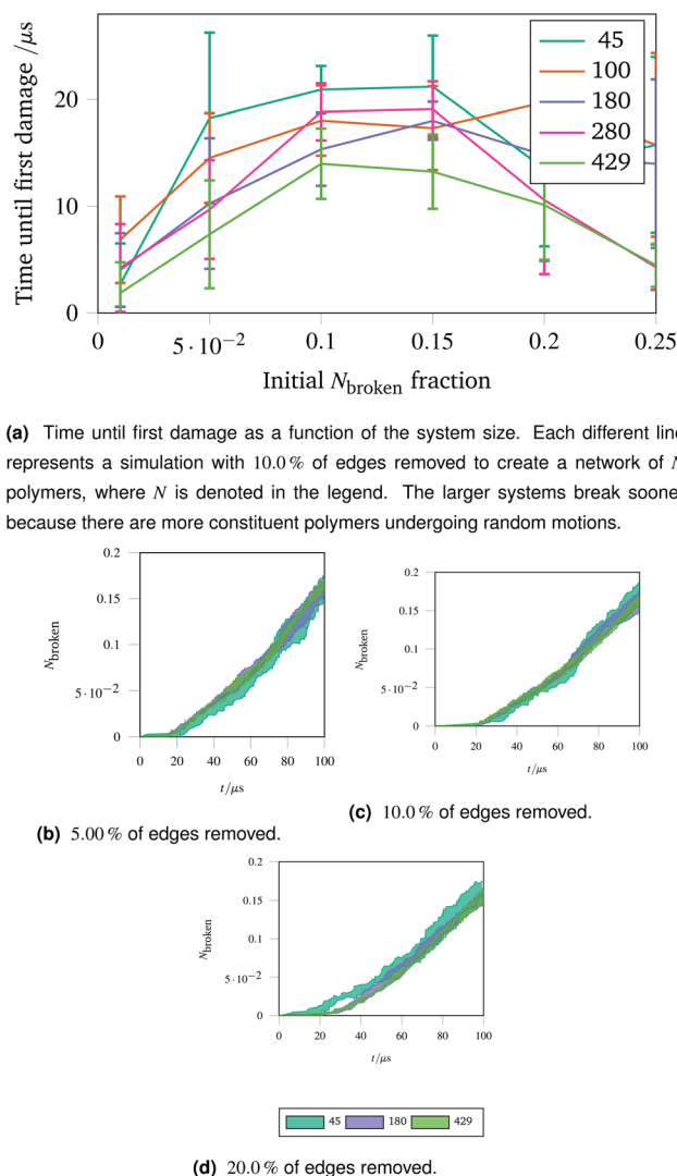
Fig. 7 Damage trajectories for systems with the same fraction of edges removed but different system sizes. The shaded area in the bottom figures shows one standard deviation of the damage trajectory as described in the caption for Fig. 4a.
