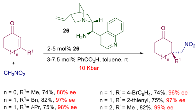
Scheme 20 Conjugate addition of nitromethane to 3-substituted cycloalkenones catalyzed by cinchonine-derived amine 26 .
