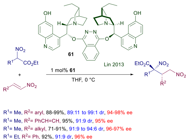
Scheme 45 Asymmetric conjugate addition of nitroesters to nitroalkenes catalyzed by bisinchona-phthalazine 61 .
