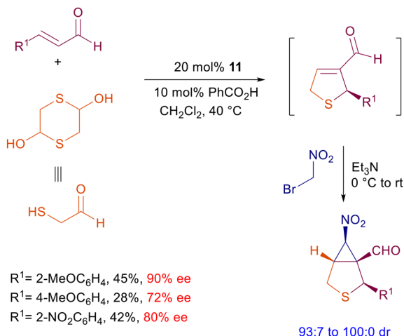
Scheme 12 Synthesis of nitrocyclopropane derivatives.
