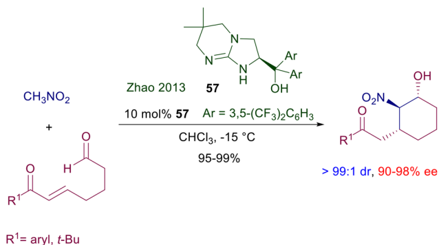
Scheme 41 Chiral bicyclic guanidine 57 as catalyst for the tandem conjugate addition/aldol condensation of nitromethane to oxoaldehydes.
