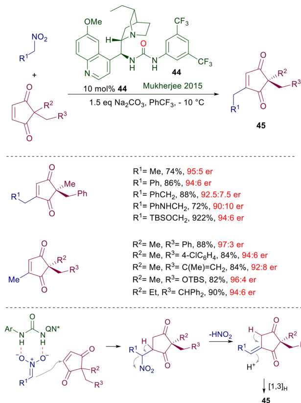
Scheme 33 Alkylative desymmetrization of cyclopentendione derivatives catalyzed by quinine-derived chiral urea 44 .
