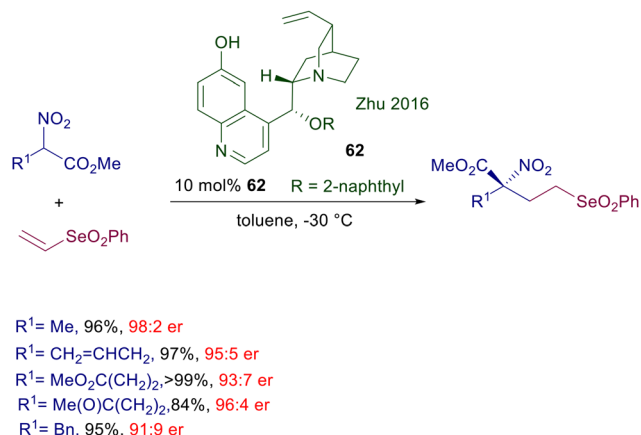
Scheme 46 Enantioselective conjugate addition of nitroesters to vinyl selenones.
