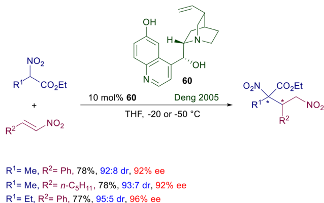
Scheme 44 Asymmetric conjugate addition of nitroesters to nitroalkenes catalyzed by cupreine 60 .
