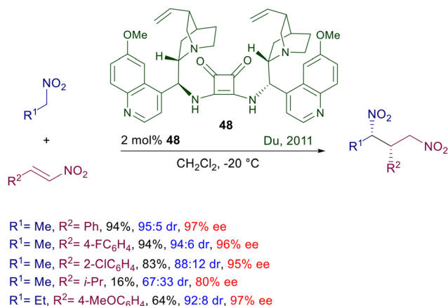
Scheme 36 Asymmetric conjugate addition of nitroalkanes to nitroalkenes catalyzed by bisquinchona-squaramide catalyst 48 .
