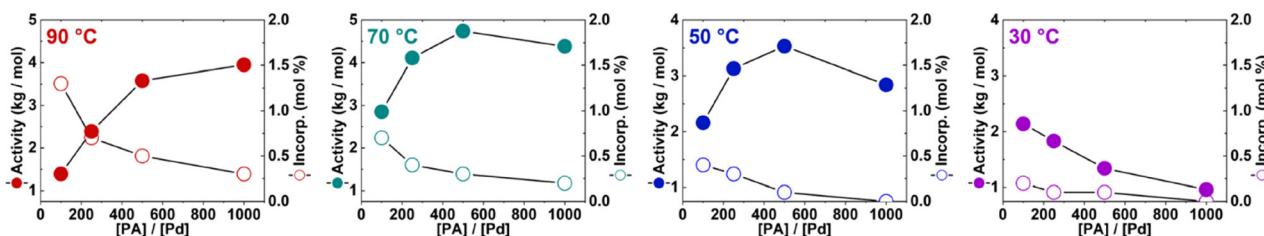
Fig. 1 Effect of the polar additive on the catalytic activities and the incorporations of the co-monomer in E-AAC copolymerization.
