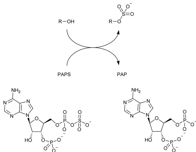
Scheme 1 Sulfotransferases add SO 3 - to hydroxyl or amino groups producing organic sulfates; PAPS functions as the donor yielding PAP as the by-product.
