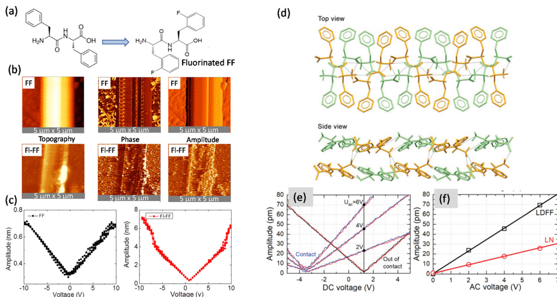
Fig. 3 Piezoelectric properties. (a) Chemical structure of FF and fluorine substituted FF (2-fluoro-L-phenylalanyl-2-fluoro-L-phenylalanine) (FI-FF). (b) Topography, phase, and amplitude images of FF and FI-FF. (c) Local DC voltage amplitude loops (piezoelectric response) from FF and FI-FF tubes at an AC voltage of 0.5 V. Reprinted with permission from ref. 65, copyright 2019, American Institute of Physics. (d) Top and side view of the bilayer of LDFF. Piezoelectric response of LDFF and LN using (e) DC voltage hysteresis loops measured at different AC voltages, and (f) AC voltage dependences on the amplitude. Reprinted with permission from ref. 15, copyright 2021, Wiley-VCH.
