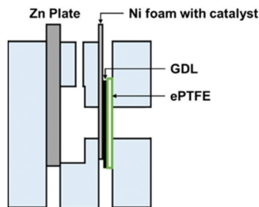
Fig. 2 A laboratory-scale ZAB for battery test showing the assembly of an air cathode comprising nickel foam with a catalyst, a GDL and ePTFE.
