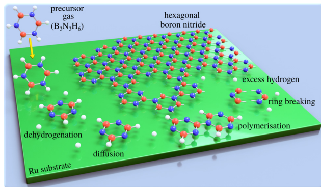
Fig. 1 Schematic illustrating the epitaxial growth of h-BN by chemical vapour deposition: a gaseous precursor (e.g. borazine, B 3 N 3 H 6 ) is brought into contact with a (hot) catalyst surface (Ru), triggering the chemical reactions such as breaking of the borazine rings and dehydrogenation, followed by the assembly of the epitaxial overlayer.
