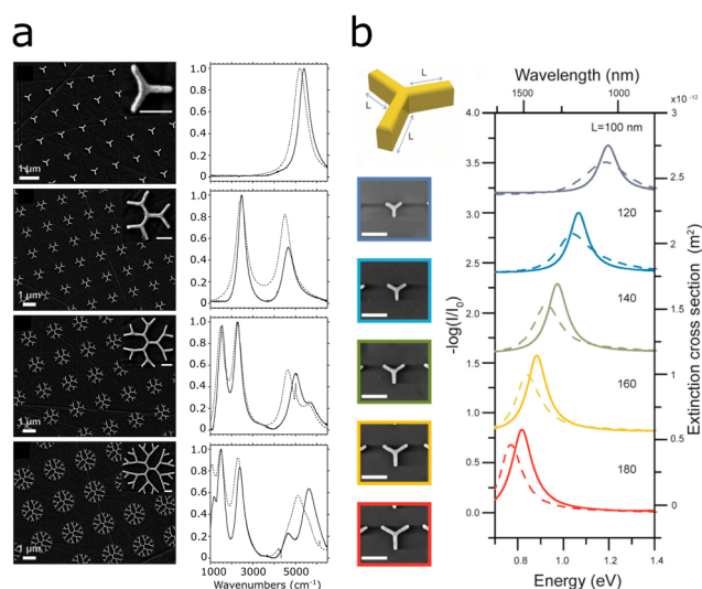
Fig. 14 Multiresonant plasmonic fractal structures. (a) SEM images of dendritic plasmonic structures of different orders (left) and corresponding normalized absorbance (right). Reprinted with permission from ref. 121. Copyright 2017 American Chemical Society. (b) Varying the resonance wavelength of first order Cayley trees by increasing the fundamental antenna length. Reprinted with permission from ref. 130. Copyright 2015 American Chemical Society.
