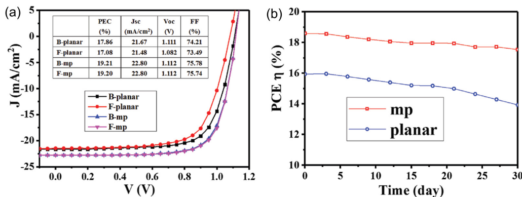
Fig. 11 (a) J - V graphs obtained of the planar SnO 2 and mp SnO 2 PSCs from under backward and forward voltage scanning. (b) PCEs of the planar SnO 2 and mp SnO 2 PSCs monitored every 3 d; the measurement was performed under AM 1.5G with input solar power P_{in} of 100 mW cm -2 . Reprinted with permission from ref. 224. Copyright 2018 John Wiley and Sons.
